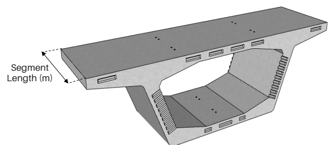
Long Section Box Girder Type Constant Depth
