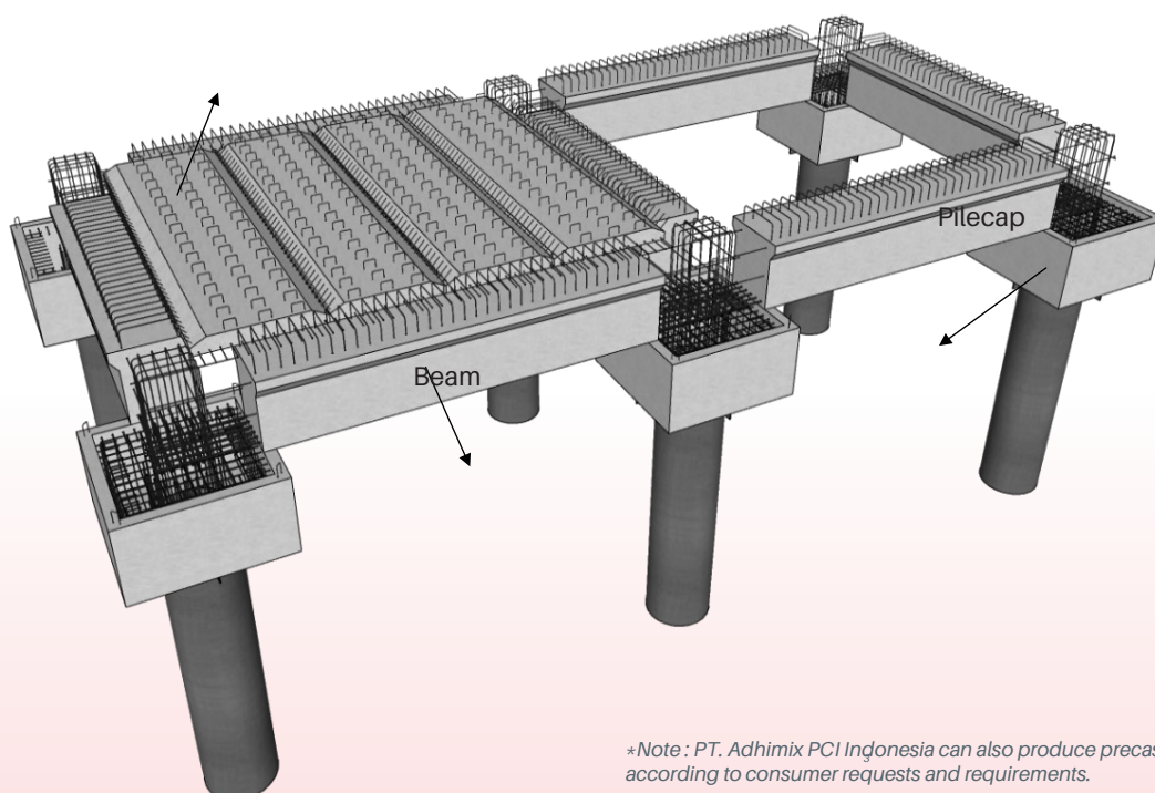
Pilecap / Head Stock
