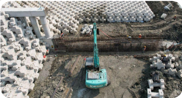
● Concrete Block Groundsill Cipamingkis River
