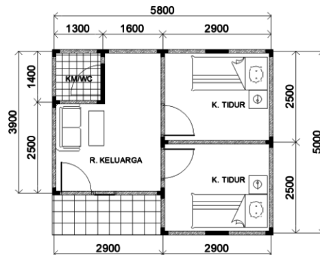
Layout House Plans - SHAPE Type 30
