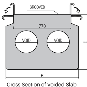
Cross Section of Voided Slab
