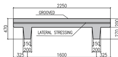
Cross Section of Double Tee Type A For Bridge Class-A ( Width of Bridge 9m )
