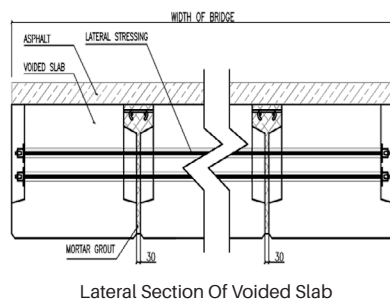
Lateral Section Of Voided Slab
